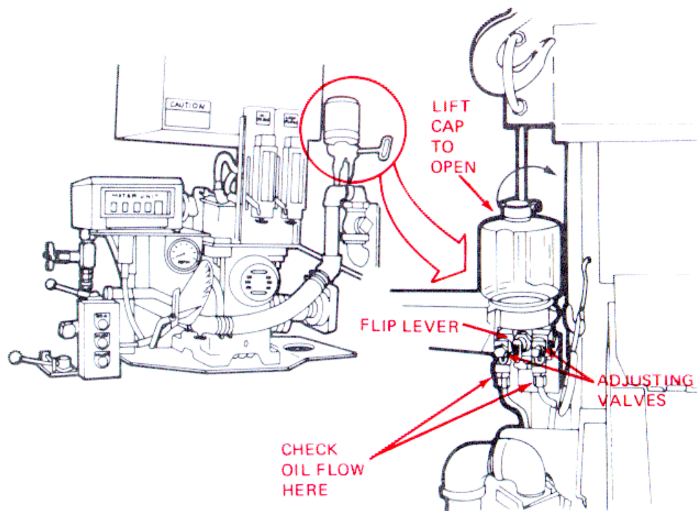
Figure 2-38. Chain Oiler
