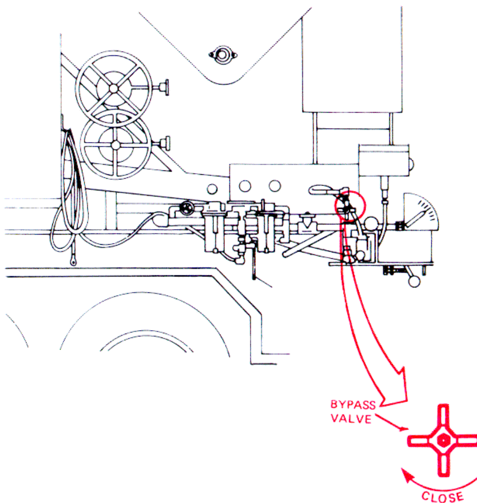
Figure 2-39. Bypass Valve.
