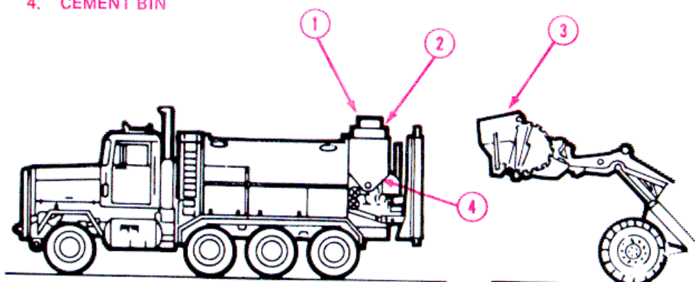
Figure 2-50. Loading the Mixer.
